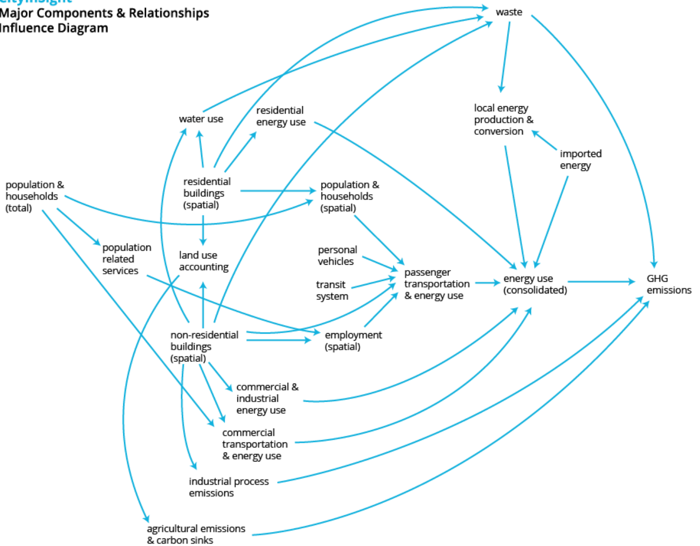
Figure 2. Representation of CityInSight's structure.
