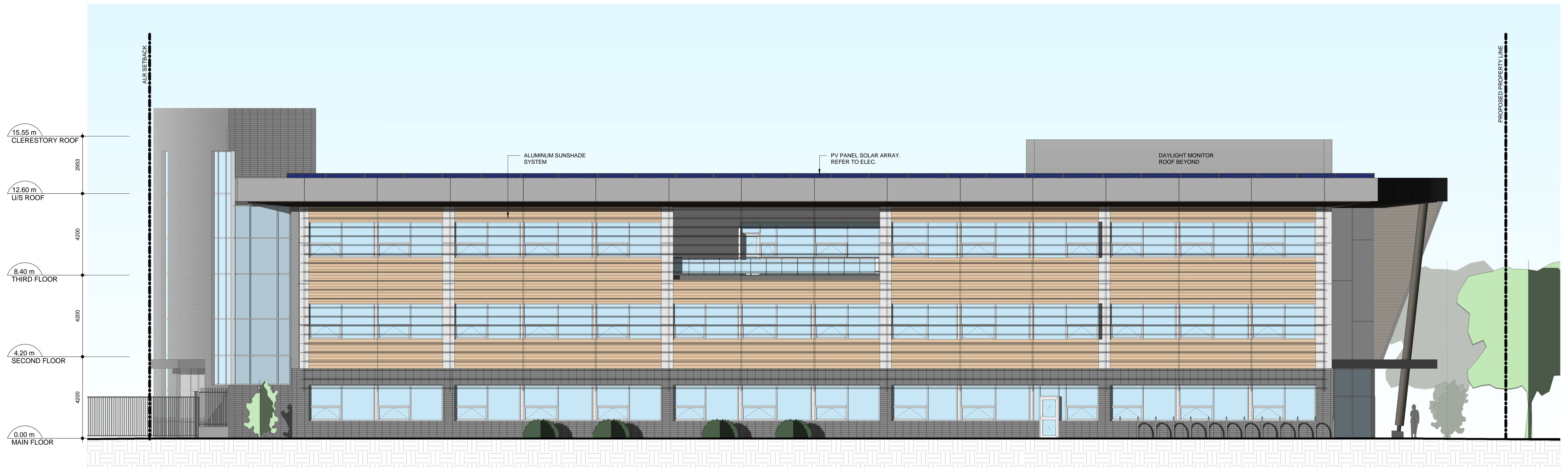
SOUTH ELEVATION 1:100
